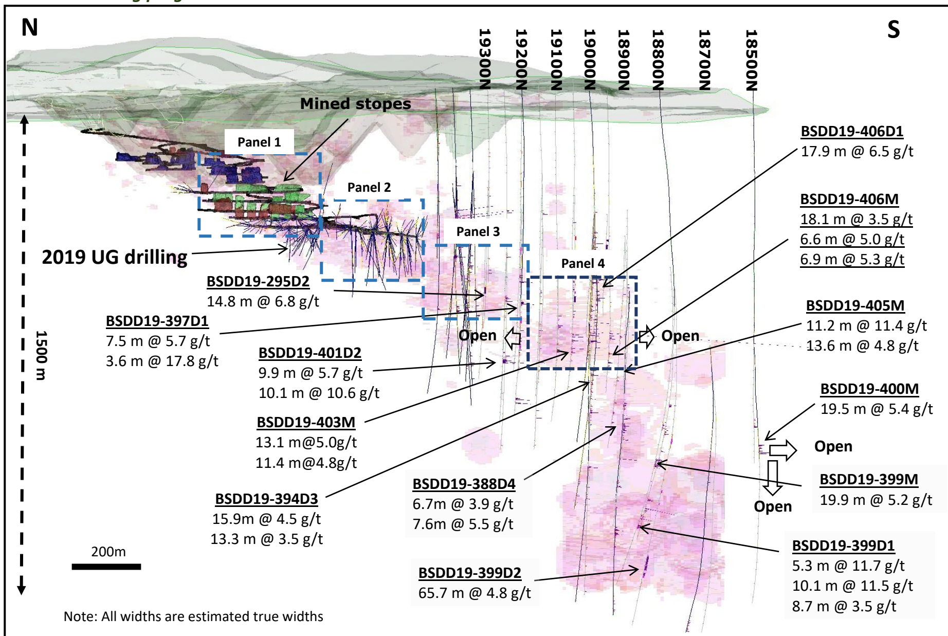
FIGURE 1: Wassa Underground: isometric view looking east showing significant results of both step out and extension drilling programs
